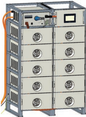
Figure 2.19 Overall diagram
