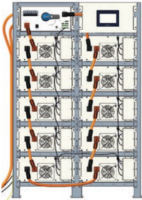
Figure 2.18 Photo after the cables are connected
