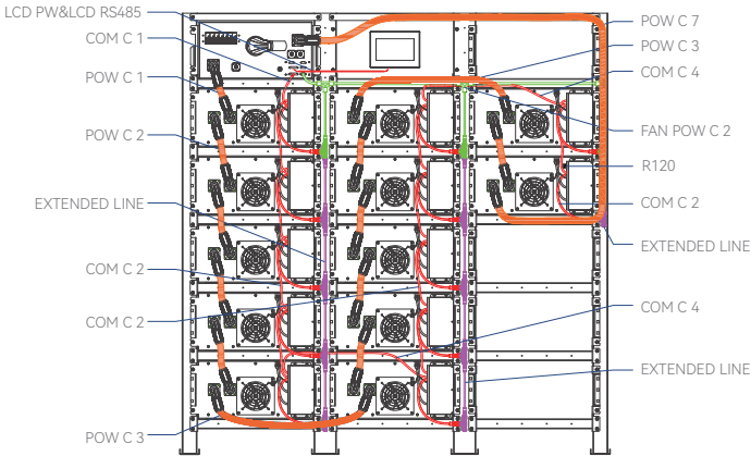
Wiring diagram
