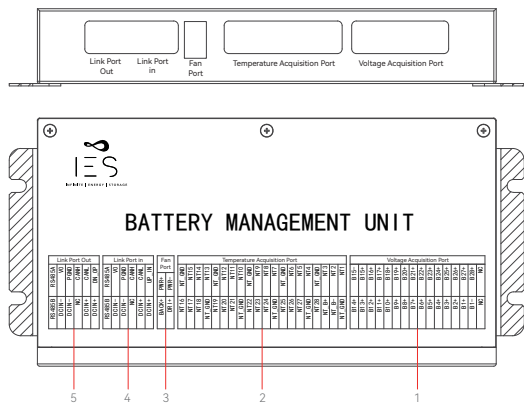
Figure 2.4 BMU photo
