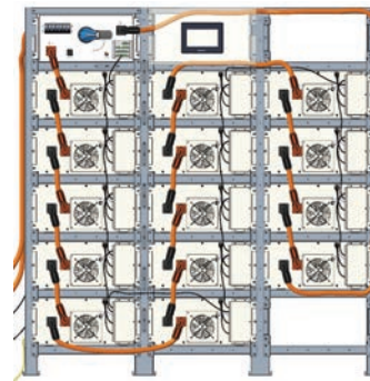
Figure 2.20 Photo after the cables are connected
