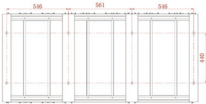
Figure 1.2 IES-R18 Rack fixed hole size drawing (unit: mm)
