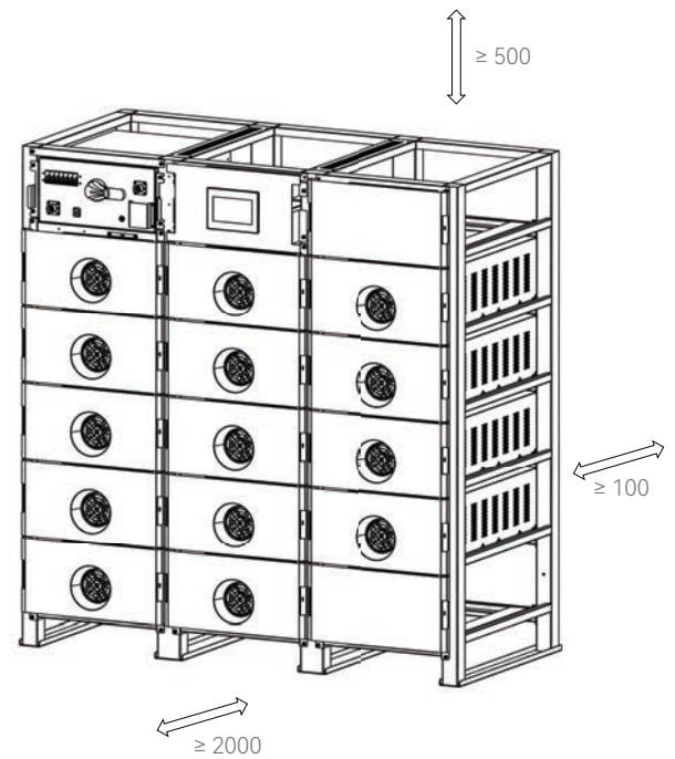
Figure 1.1 Schematic diagram of reserved space
