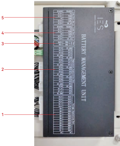
Figure 2.4 BMU photo
