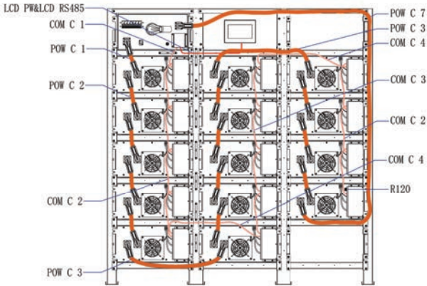
Wiring diagram
