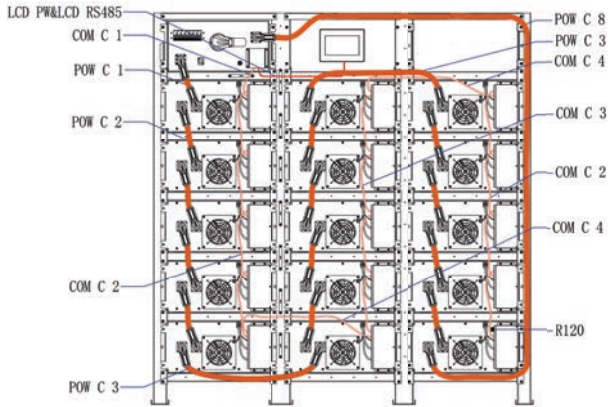
Wiring diagram
