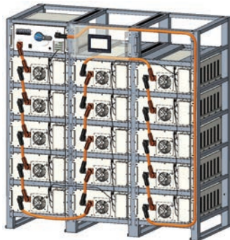
Schematic diagram of power line
