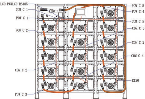
Wiring diagram
