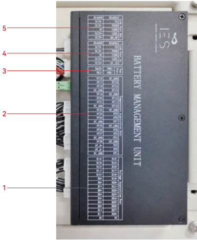
Figure 2.4 BMU photo
