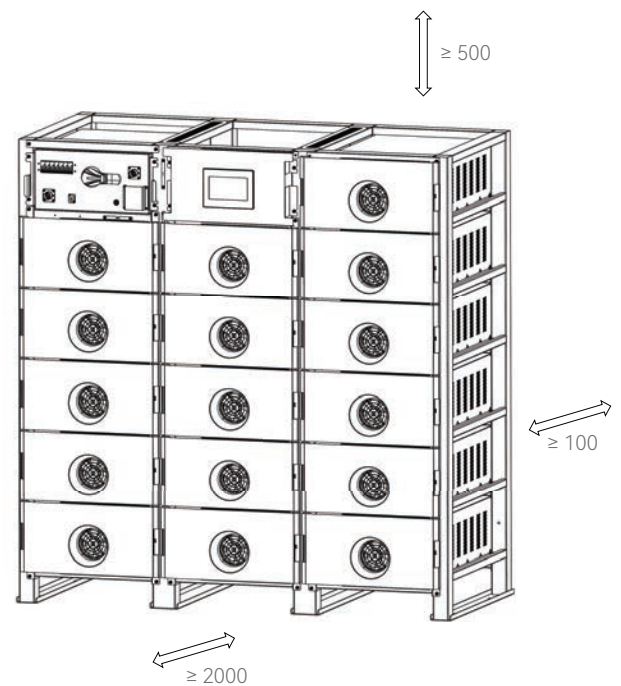
Figure 1.1 Schematic diagram of reserved space
